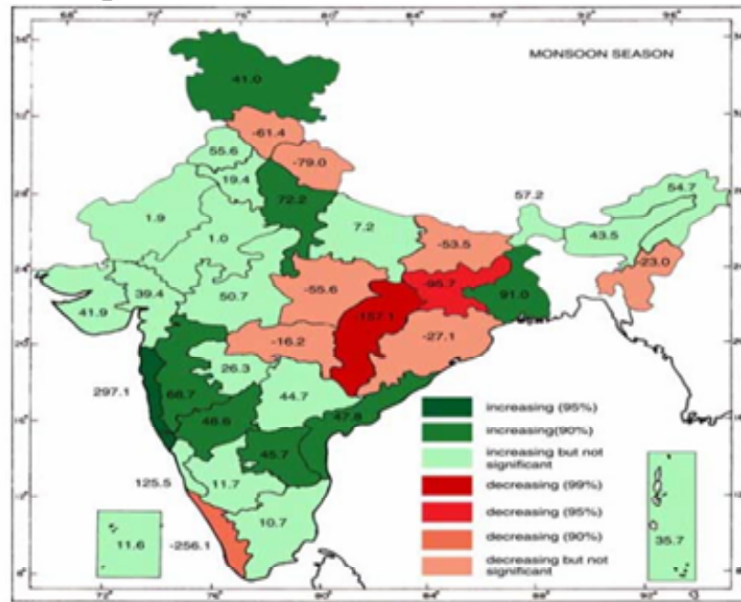
Trends in Regional Distribution of Rainfall
