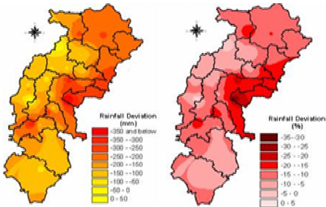
Rainfall decrease during the period 1951-2000 as compared to normal (1901-50) values in Chhattisgarh
